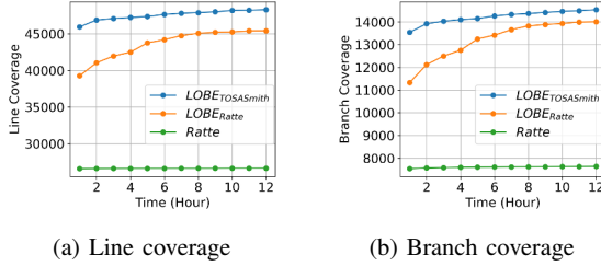
Fig. 6: Coverage information over a 12-hour budget
