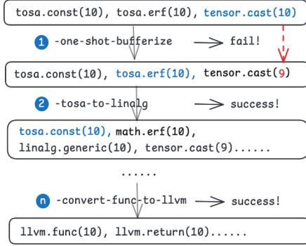
(a) An MLIR program
